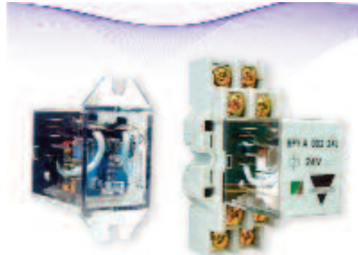
Blade Pin 16A SPDT / 10A DPDT LED Indication (Plug Mount Only)
