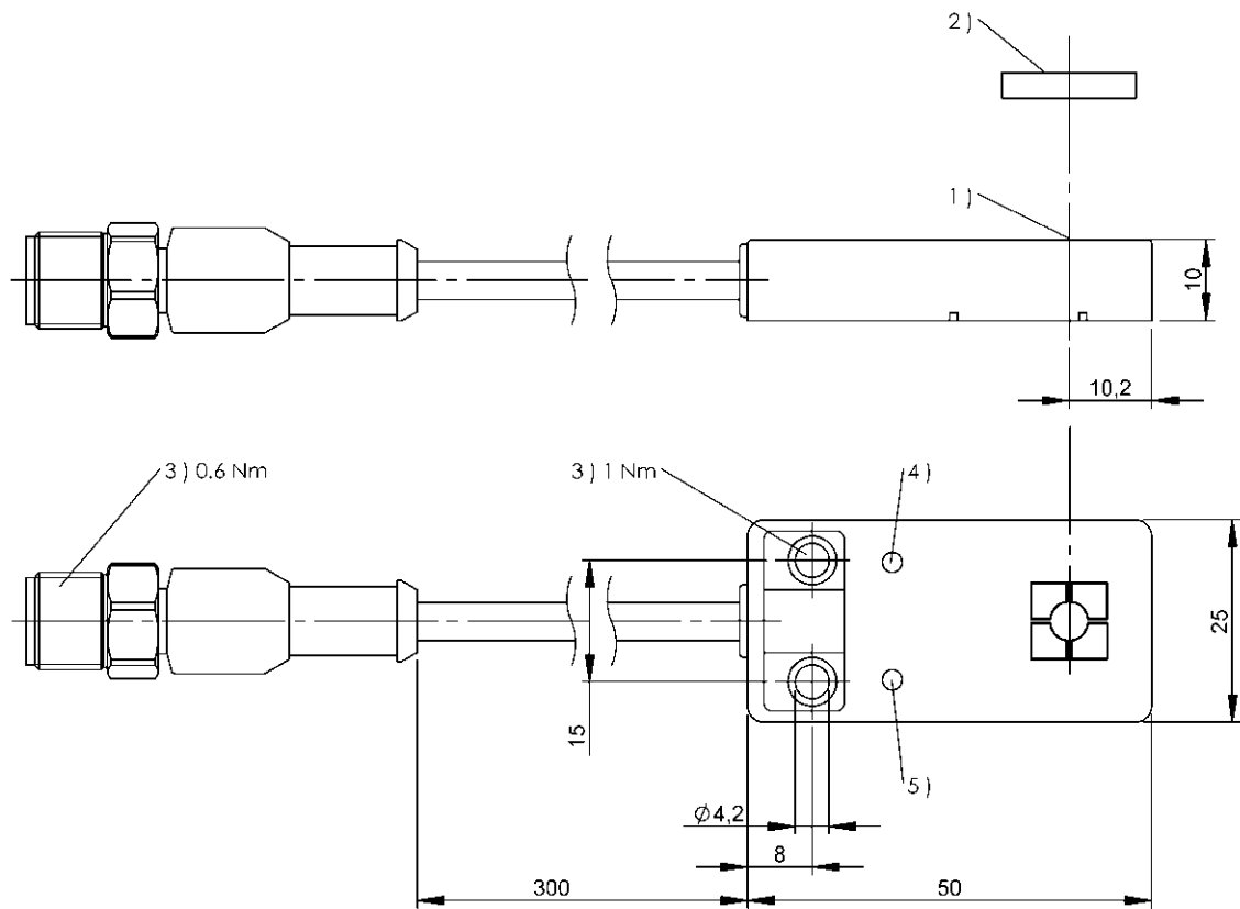
1) Sensing surface, 2) Data carrier, 3) Tightening torque, 4) LED function indicator, 5) LED function indicator
