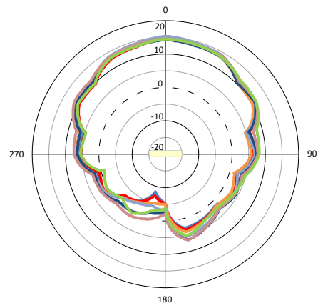
V-pol Azimuth
