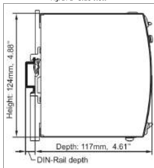
Fig. 21-2 Side view
